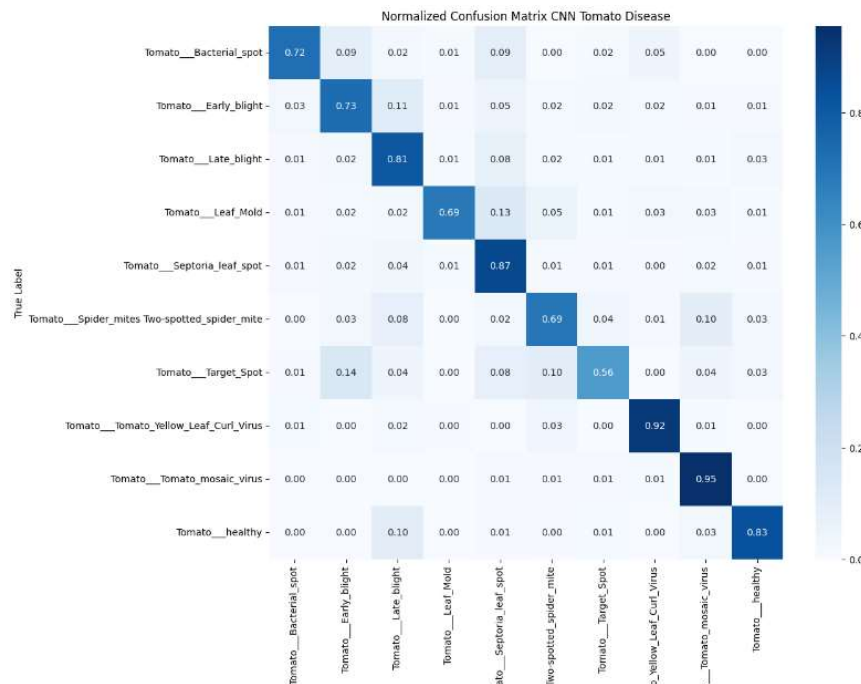
Gambar 3. Normalized confusion matrix sepuluh kelas daun tomat
